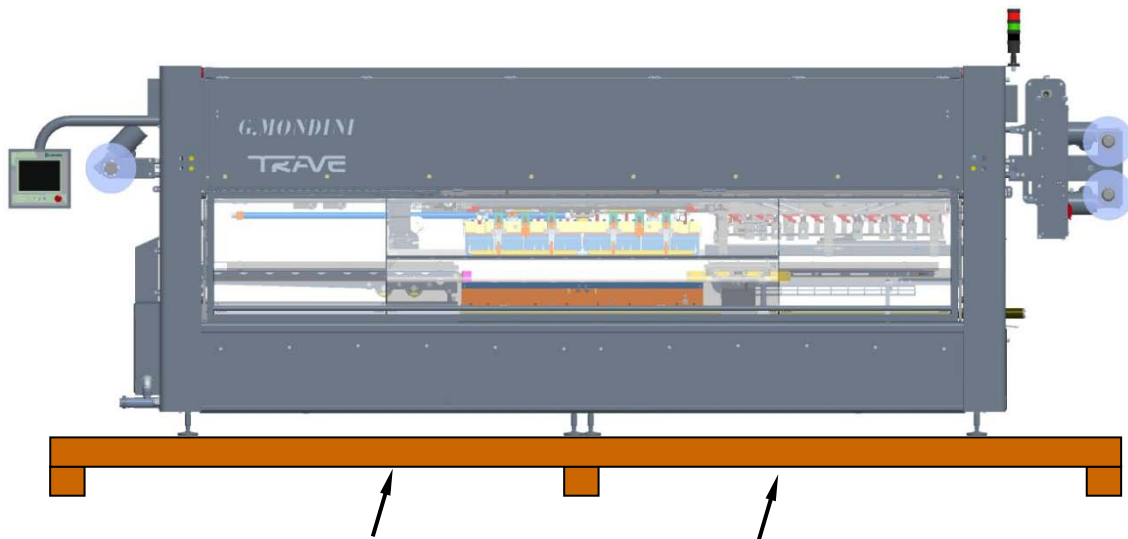
Figure 4-1: Lifting using a forklift truck.
